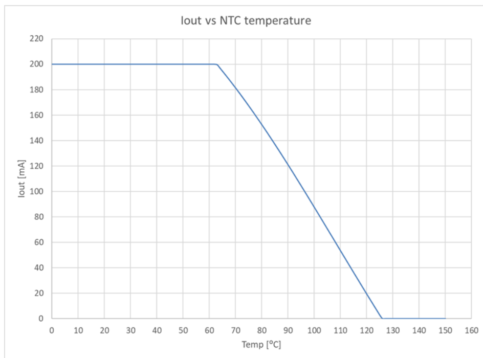
Figure 18. Simulated I_{\text{OUT}} vs. NTC temperature
