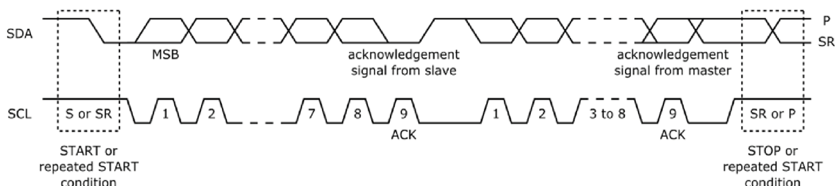
Figure 21. Bit transfer
