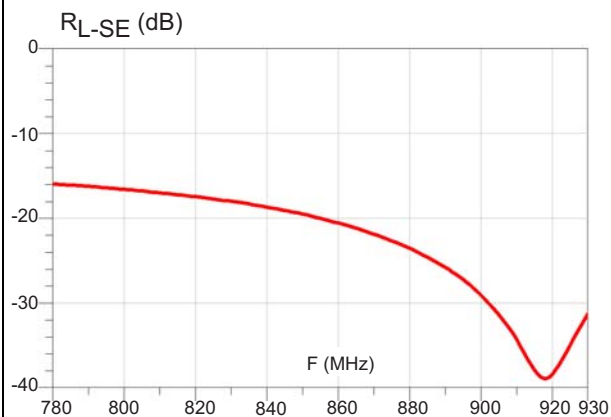
Figure 4. Return loss single-ended
