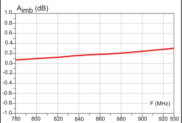
Figure 7. Amplitude imbalance
