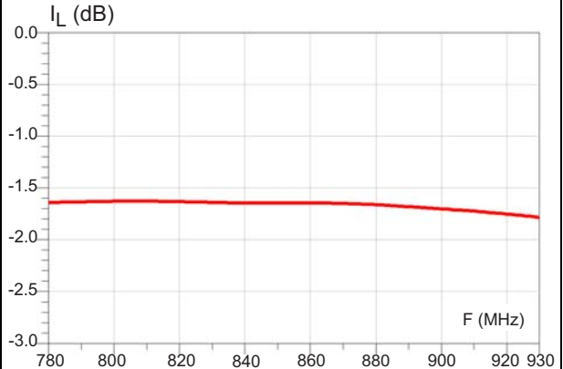
Figure 3. Insertion loss in band
