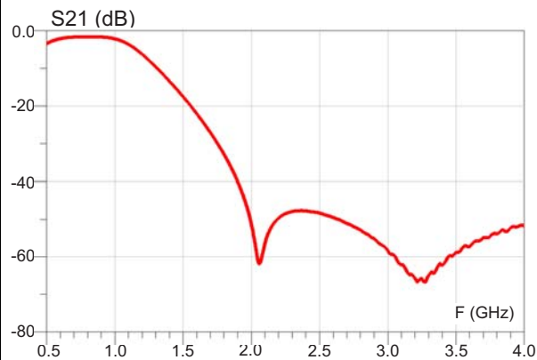
Figure 2. Transmission (S21)
