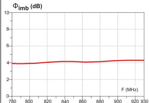
Figure 6. Phase imbalance
