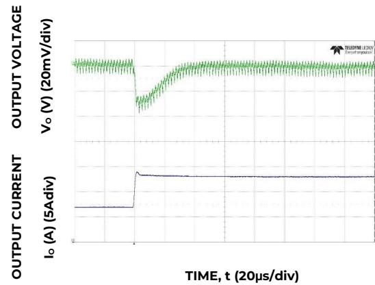
Figure 16. Transient Response to Dynamic Load Change from 50% to 100% at 12V in , C out =8x47μF+2x330μF C Tune =1.8nF, R Tune =300Ω
