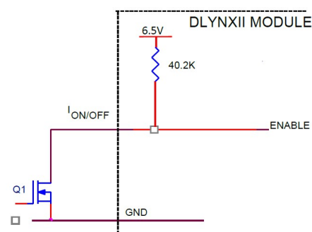
Figure 39. Circuit configuration for using positive On/Off logic.
