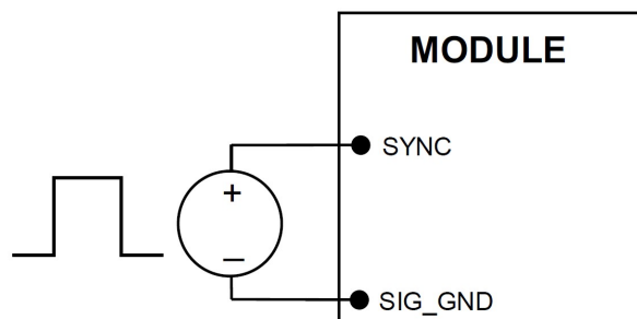
Figure 45. External source connections to synchronize switching frequency of the module. Measuring Output Current, Output Voltage and Temperature.
