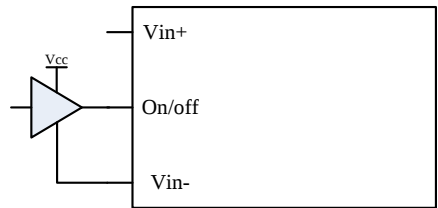
Figure 6. Control with logic circuit
