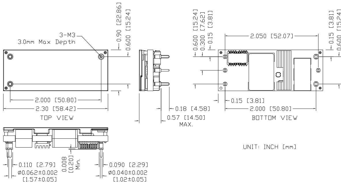
Figure 15. ORCY-F0S10B Outline
