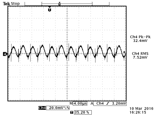
Figure 11. Ripple and noise, 54 VDC input, 500 W output, T_a = 25^\circ\text{C} , with C_{out} = 500\ \mu\text{F} (50% ceramic, 50% 50% Oscon caps)
