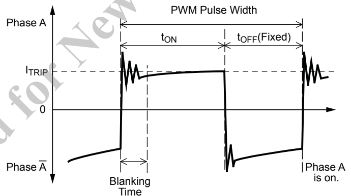
Figure 7. Sensex pin waveform during PWM control
