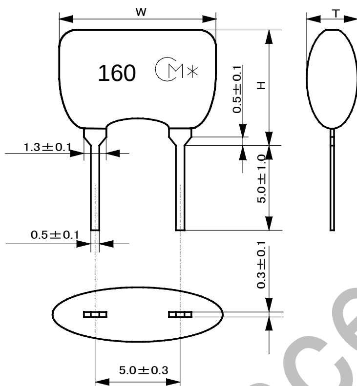
Figure 1. Dimensions (CSALF16M0X55-B0)
