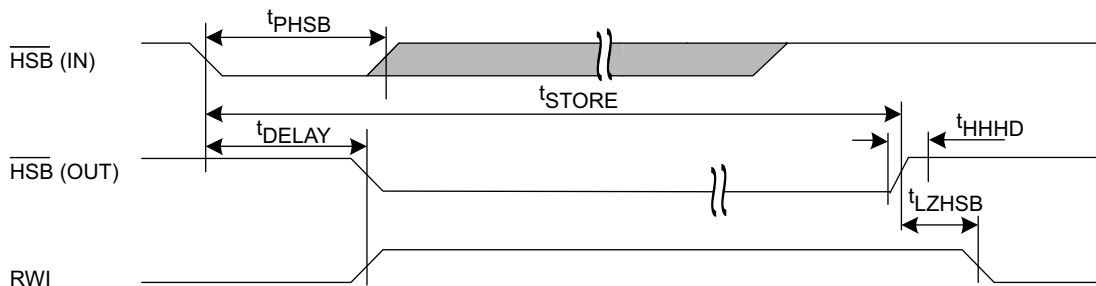
Figure 14. Hardware STORE Cycle [49]
