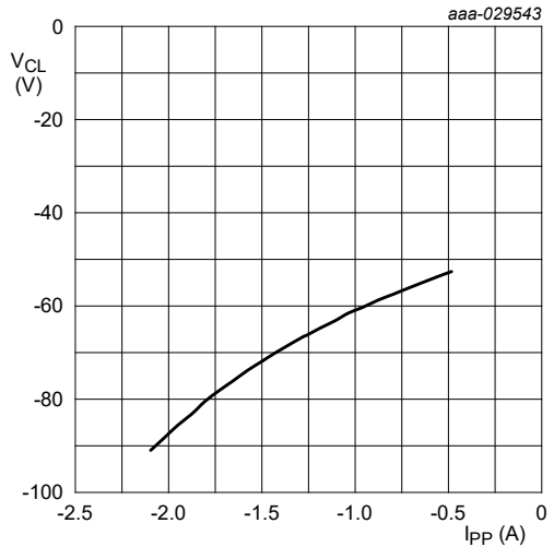
Fig. 6. Negative clamping voltage (8/20 \mu\text{s} pulse); typical values
