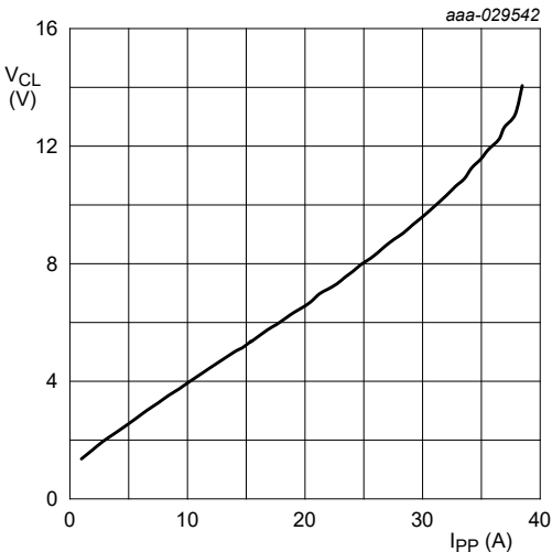
Fig. 5. Positive clamping voltage (8/20 \mu\text{s} pulse); typical values
