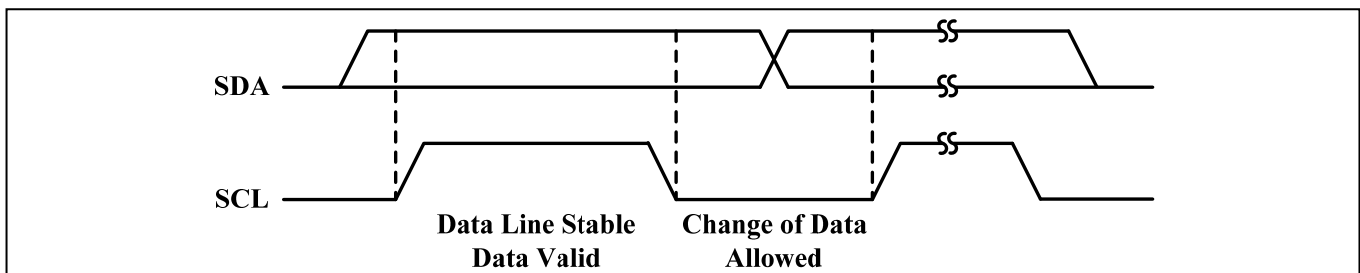
Figure 3 Bit transfer
