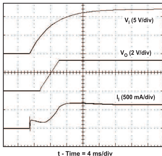
Figure 11. Power-Up Waveform
