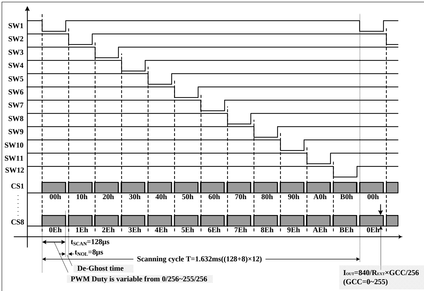
Figure 12 Scanning Timing
