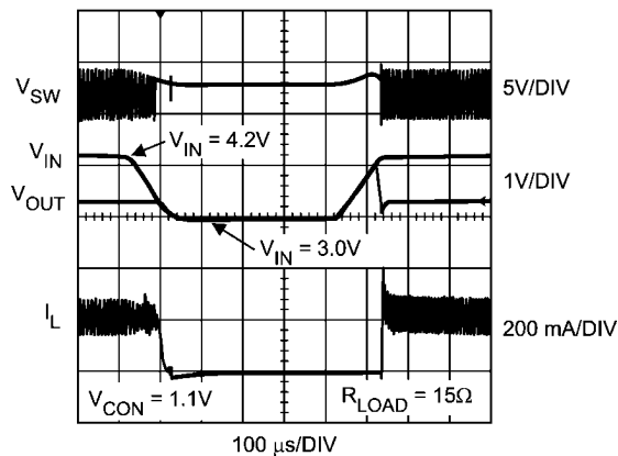
Automatic Bypass Operation ( V_{IN} = 4.2V to 3.0V )
