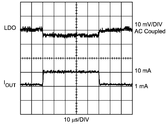
LDO Load Transient Response ( C_{OUT} = 1 \mu F )
