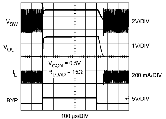
Forced Bypass Operation ( V_{IN} = 3.0V )
