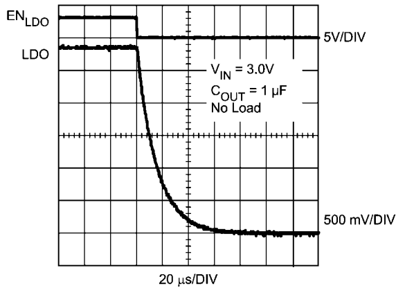
LDO Turn OFF ( EN_{LDO} = High to Low)
