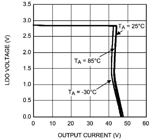
LDO Voltage vs Output Current ( V_{IN} = 3.6V )
