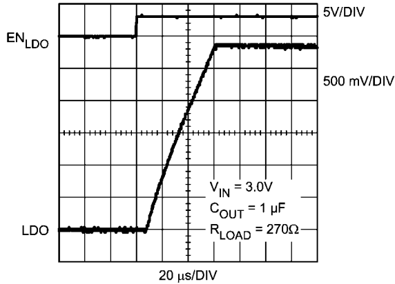
LDO Turn ON ( EN_{LDO} = Low to High)
