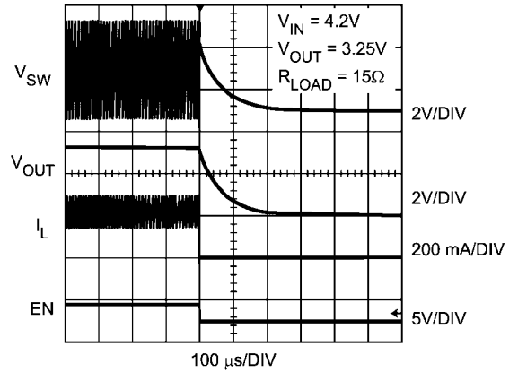
PWM Shutdown Response ( V_{CON} = 1.08V )
