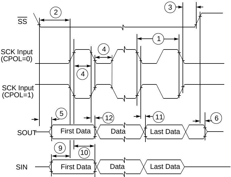
Figure 42. DSPI classic SPI timing—slave, CPHA = 0
