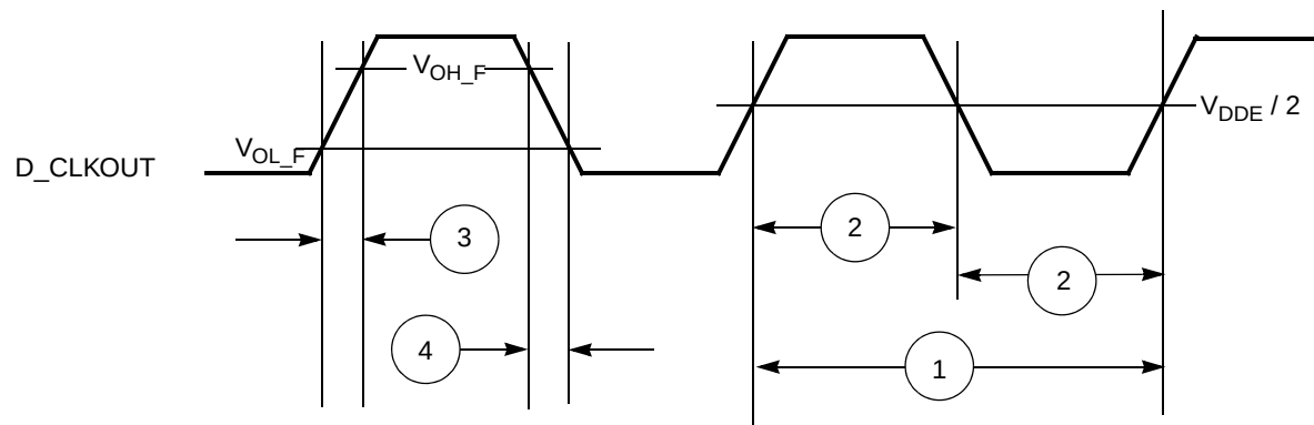
Figure 55. D_CLKOUT timing
