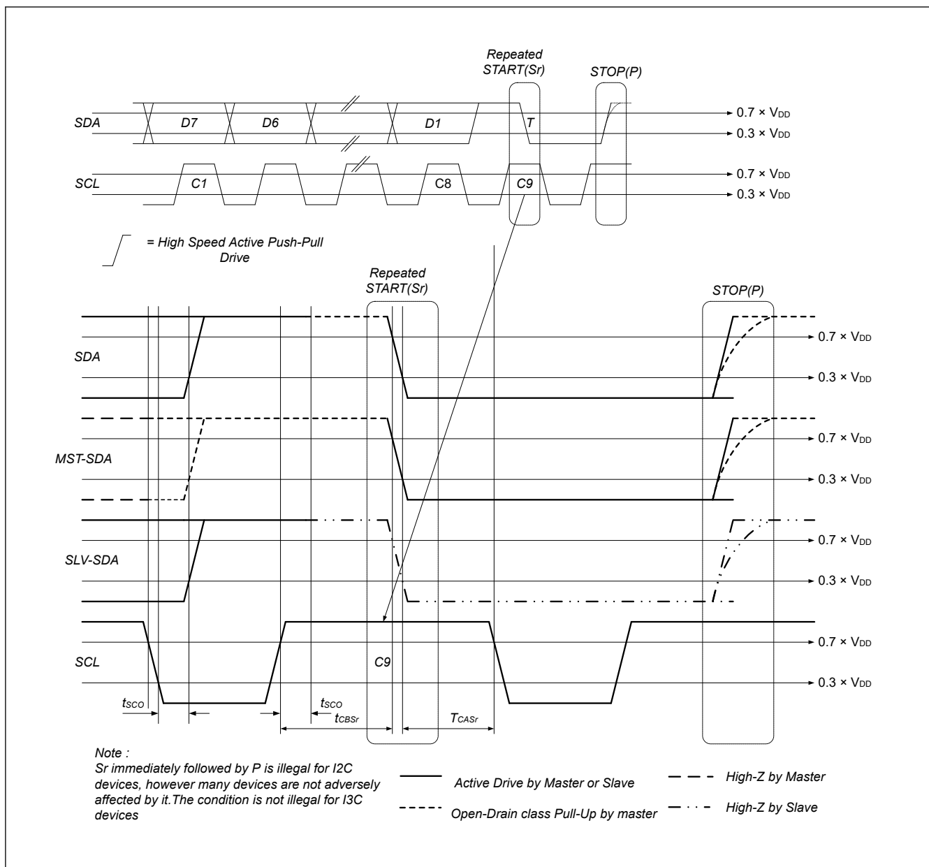
Figure 2.43 T-Bit When Master Ends Read with Repeated START and STOP
