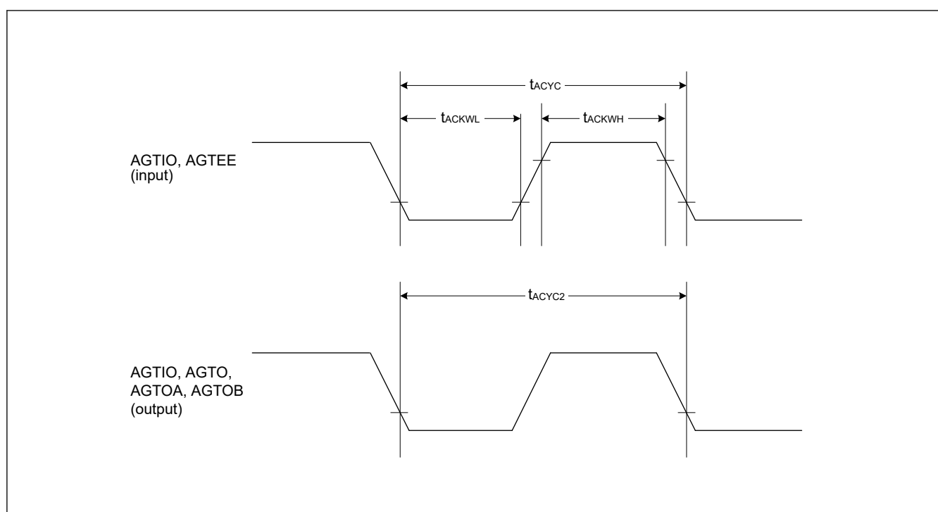
Figure 2.17 AGTAGTW I/O timing
