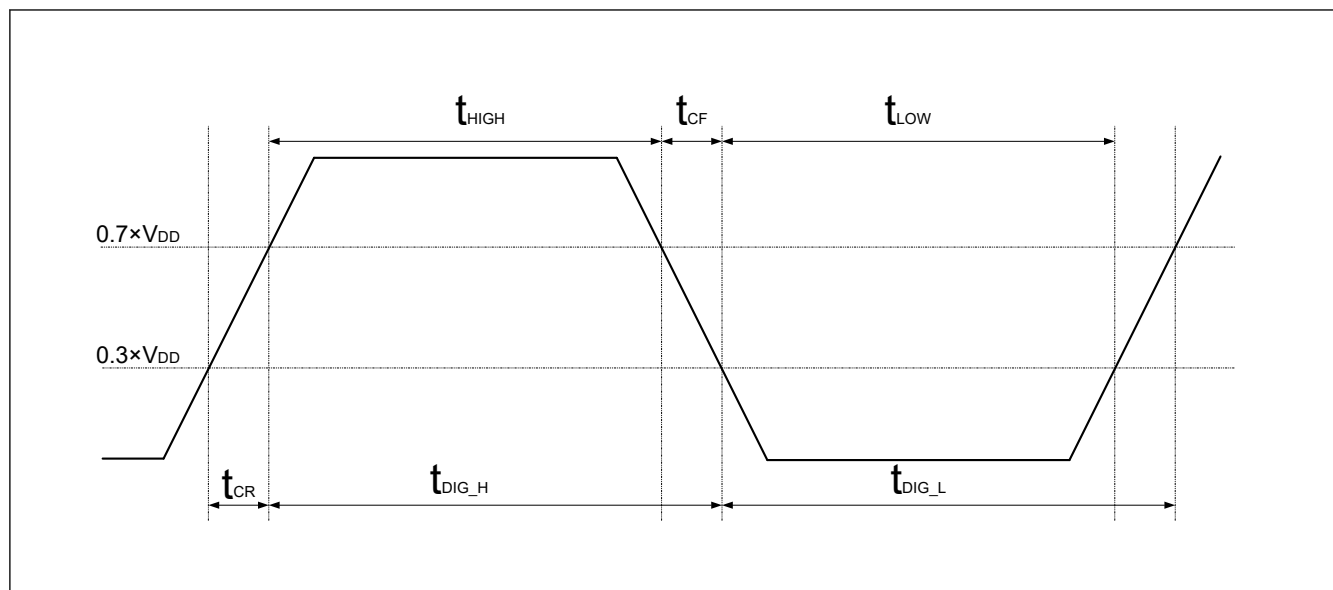
Figure 2.36 t_{DIG\_H} and t_{DIG\_L}
