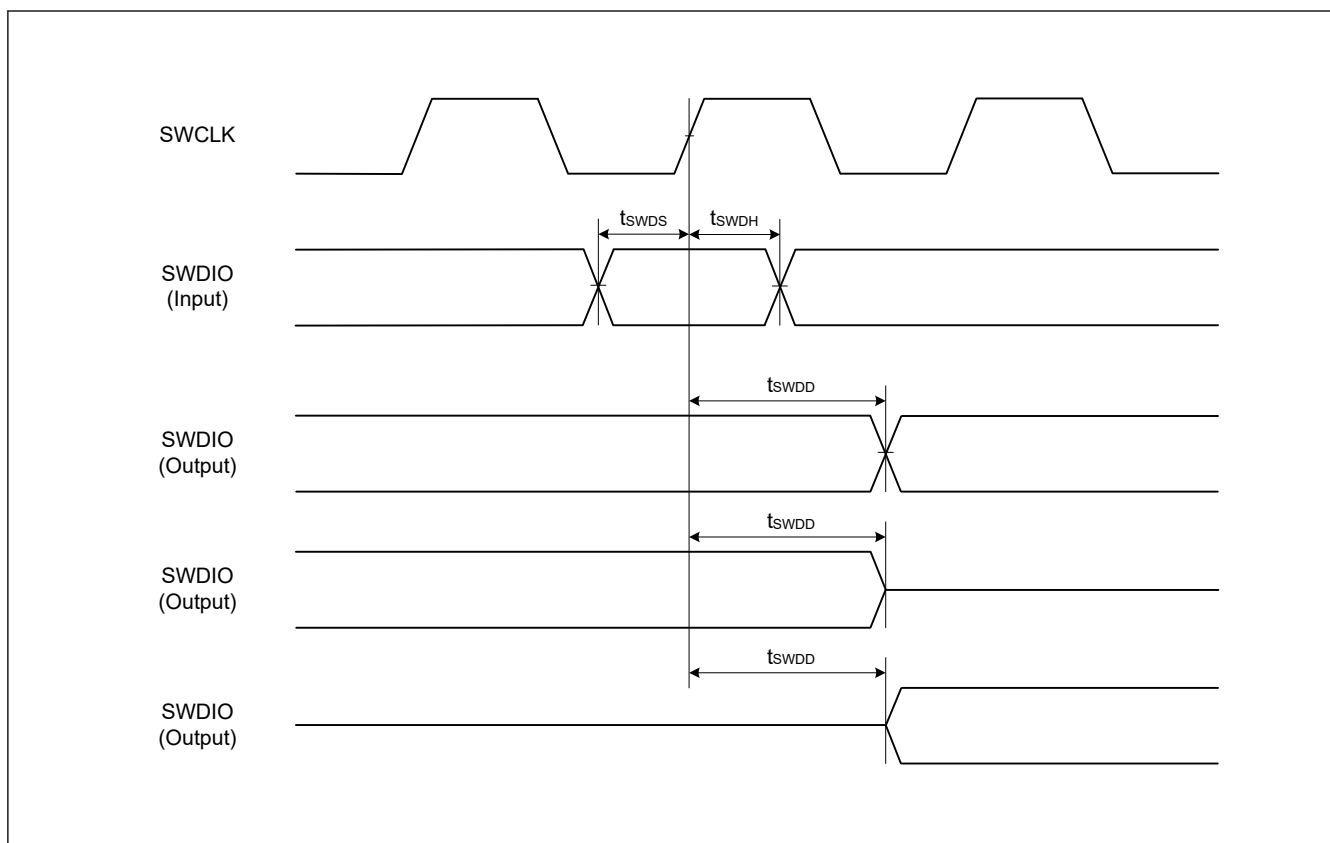
Figure 2.55 SWD input/output timing
