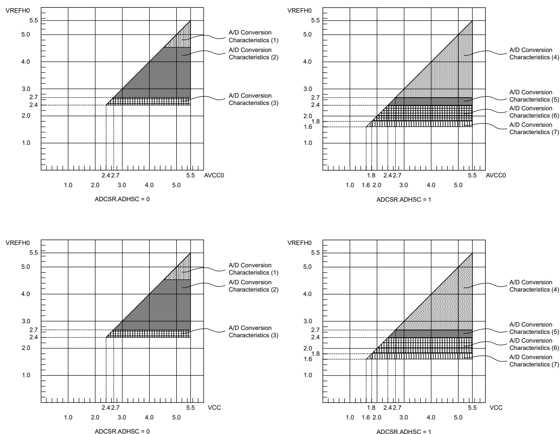
Figure 2.46 VCC0 to VREFH0 voltage range
