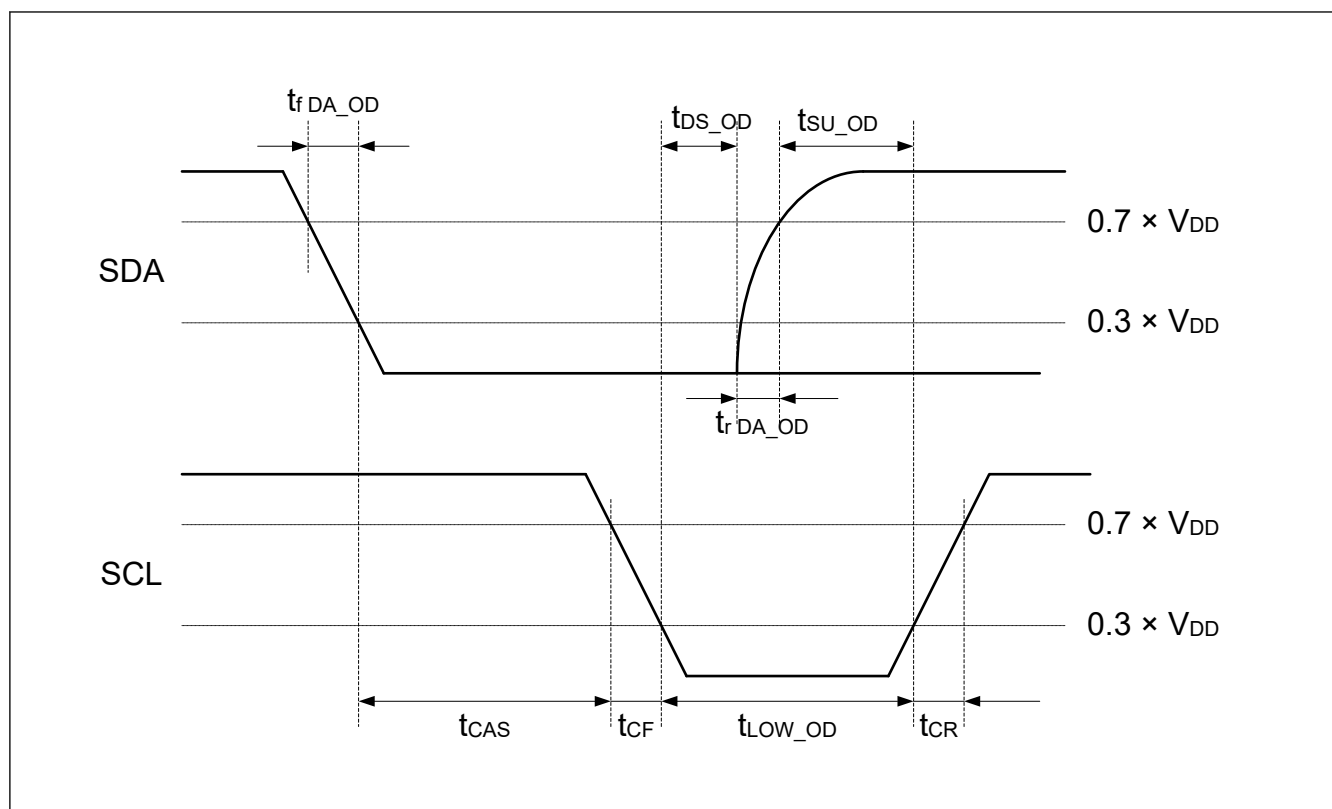
Figure 2.38 I3C START condition Timing
