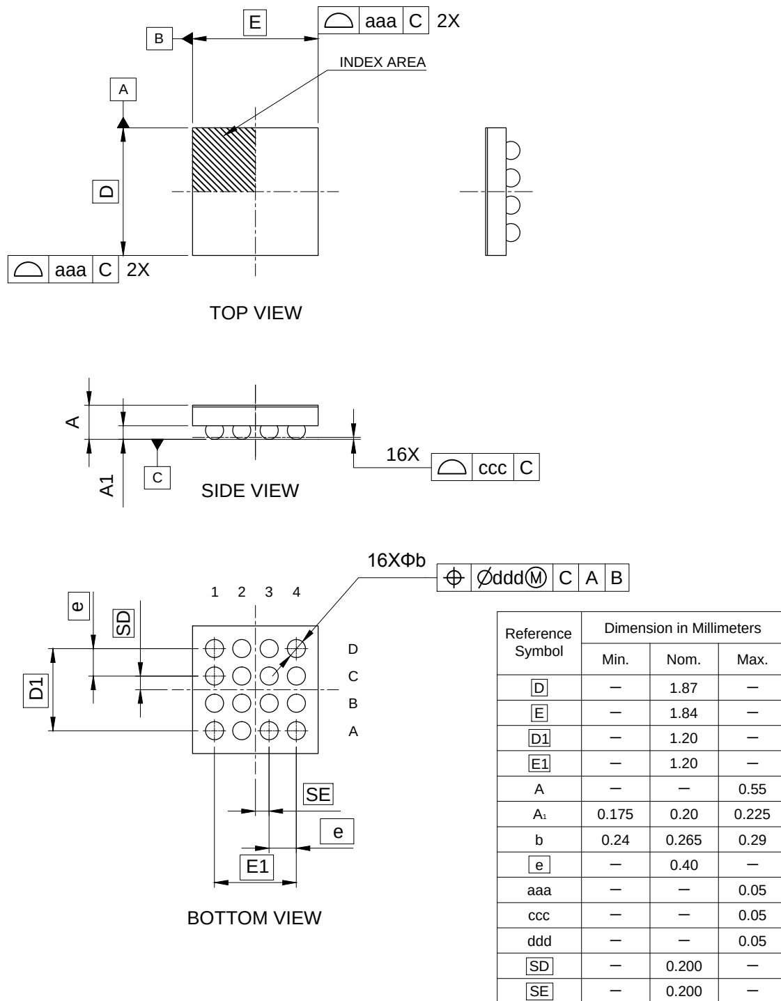
Figure A2.3 WLCSP 16-pin
