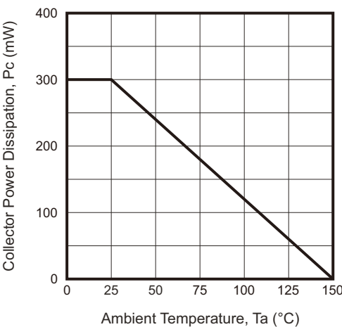
Fig.7 - Collector Power Derating Curve
