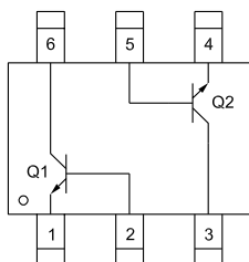
CMKT3904 (NPN/NPN)
