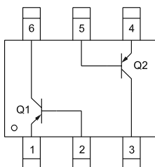
CMKT3906 (PNP/PNP)
