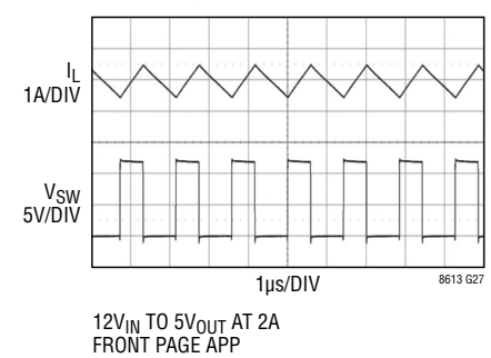
Switching Waveforms
