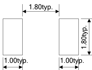
Recommended Pad Layout (mm)
