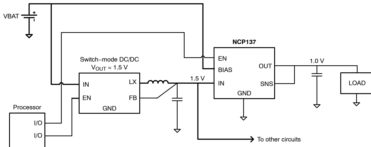
Figure 4. Typical Application: Low-Voltage DC/DC Post-Regulator with ON/OFF Functionality
