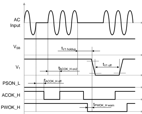
Figure 27. AC short dips
