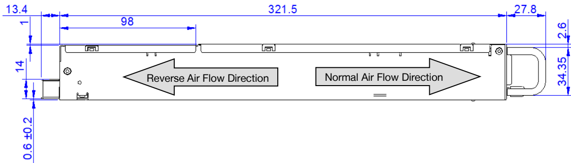
Figure 43. Side View 1
