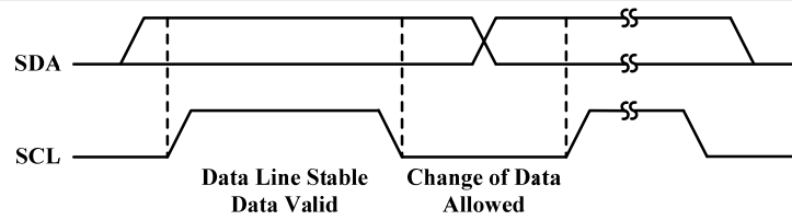
Figure 4 Bit Transfer
