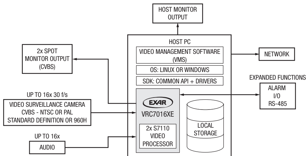
Figure 1. Typical Application
