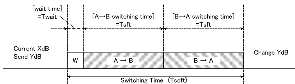
Figure 11. Micro step volume switching time
