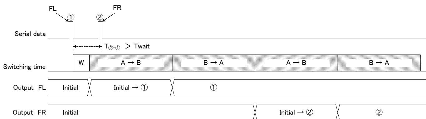
Figure 15. The operation during multi-channels (Lch, Rch) data transmission (larger than T_{wait} interval).
