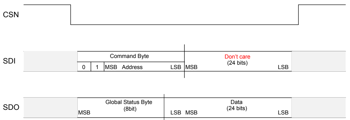
Figure 16. SPI read operation
