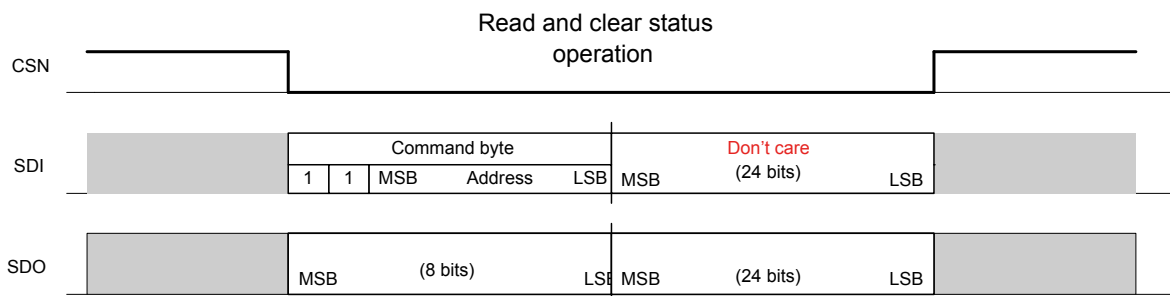
Figure 18. SPI read device information
