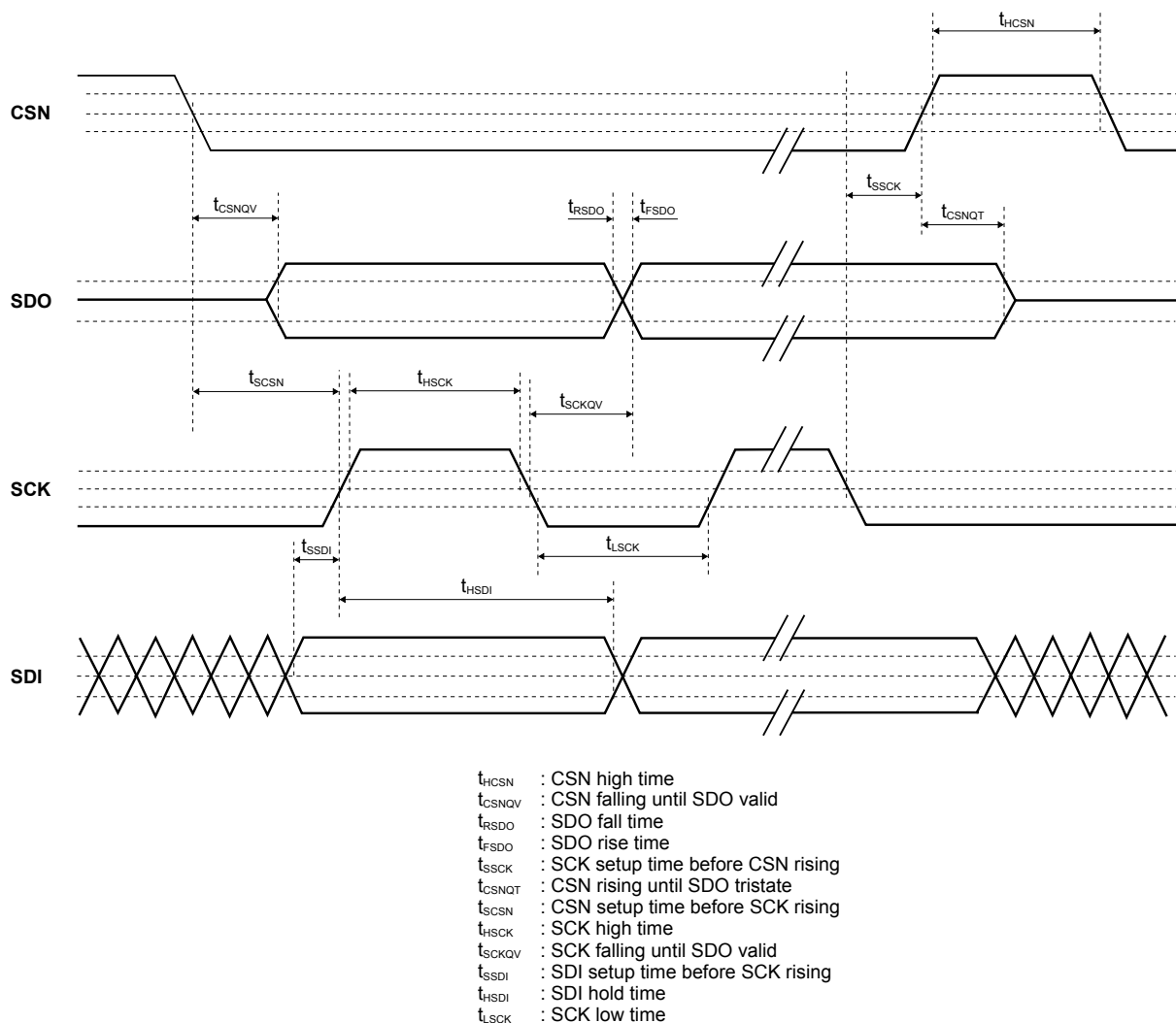
Figure 3. SPI specification: timing waveforms
