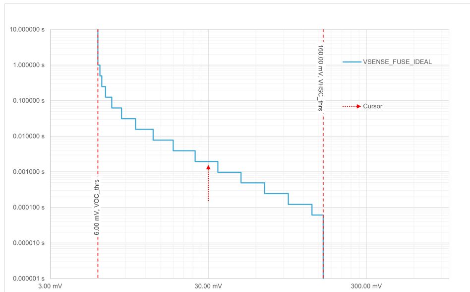
Figure 5. eFuse I 2 -t typical curve (VOC_thrs minimum - VHSC_thrs maximum)
