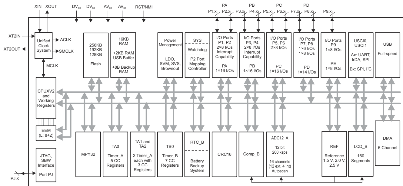
Figure 4-2. Functional Block Diagram – MSP430F6635, MSP430F6634, MSP430F6633
