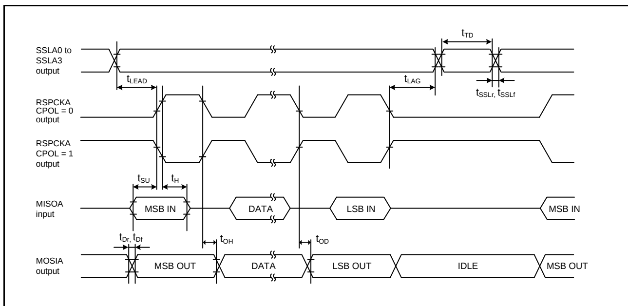
Figure 2.57 RSPI Timing (Master, CPHA = 0) (Bit Rate: PCLKB Division Ratio Set to a Value Other Than 1/2)
