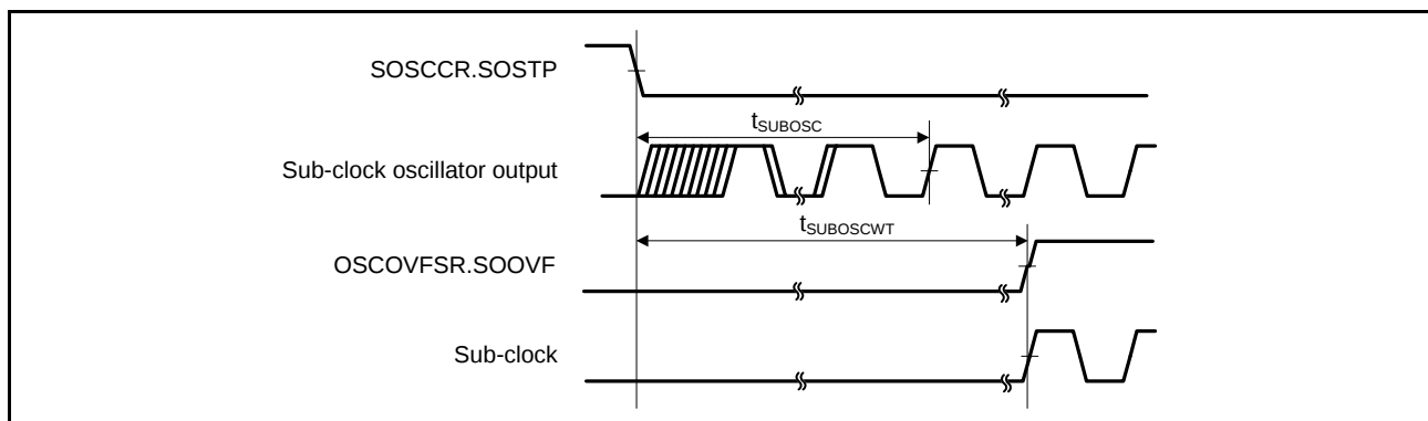
Figure 2.11 Sub-Clock Oscillation Start Timing
