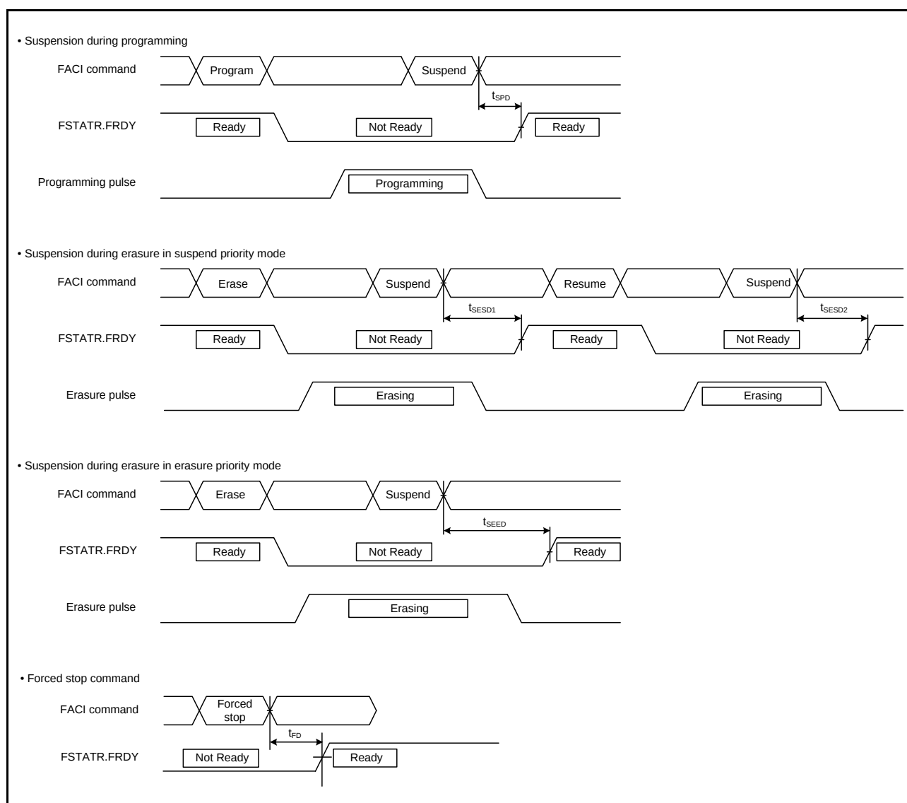
Figure 2.96 Flash Memory Programming/Erasure Suspension Timing
