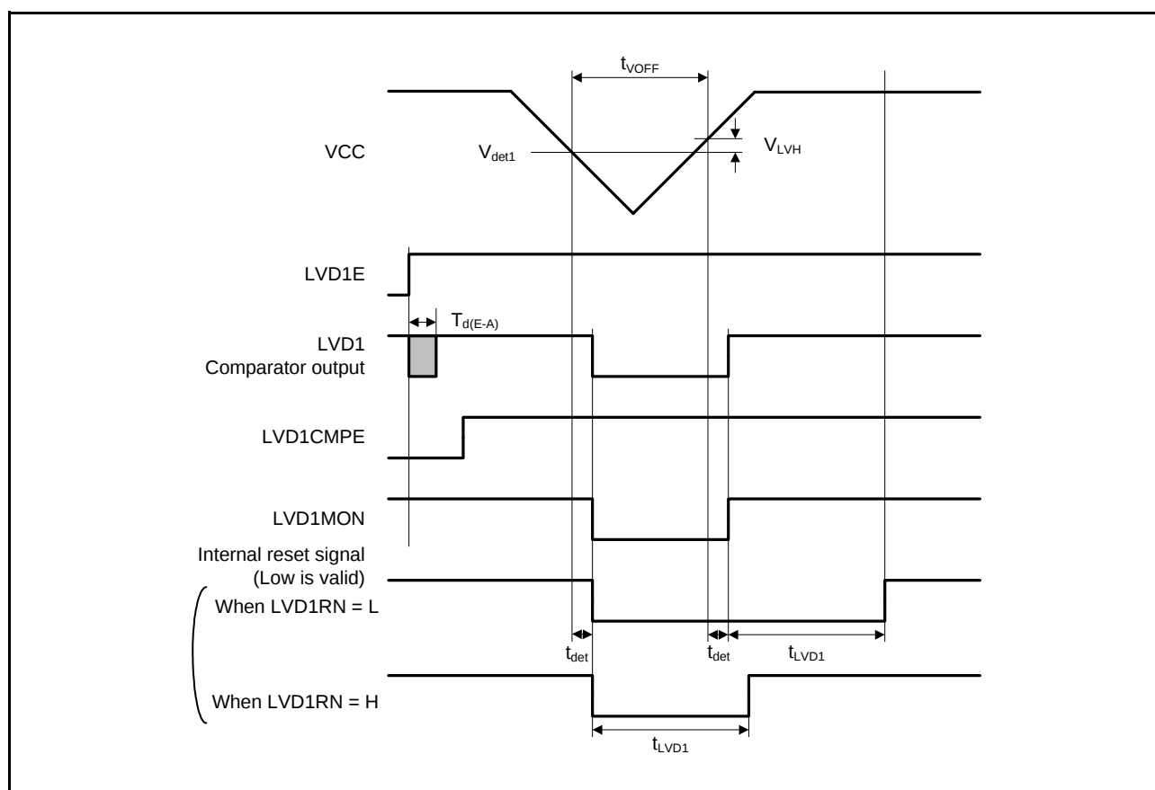
Figure 2.92 Voltage Detection Circuit Timing ( V_{det1} )
