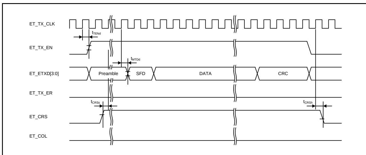
Figure 2.77 MII Transmission Timing (Normal Operation)
