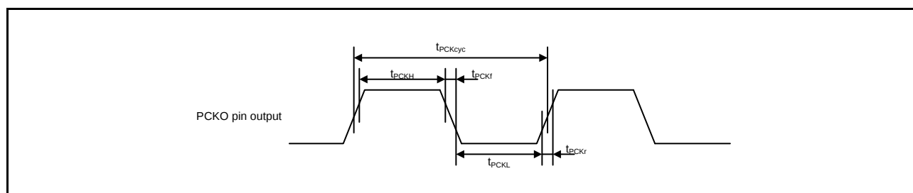
Figure 2.83 PDC Output Clock Timing
