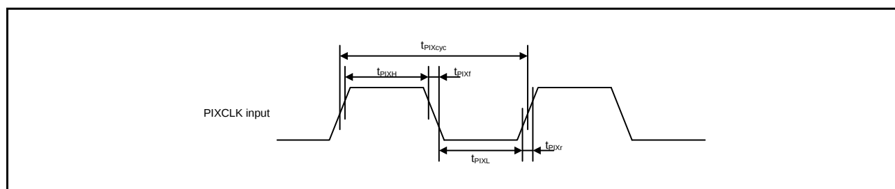
Figure 2.82 PDC Input Clock Timing
