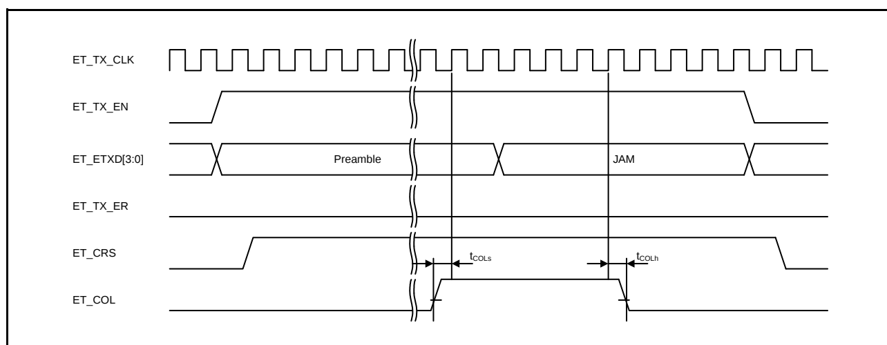
Figure 2.78 MII Transmission Timing (Conflict Occurrence)
