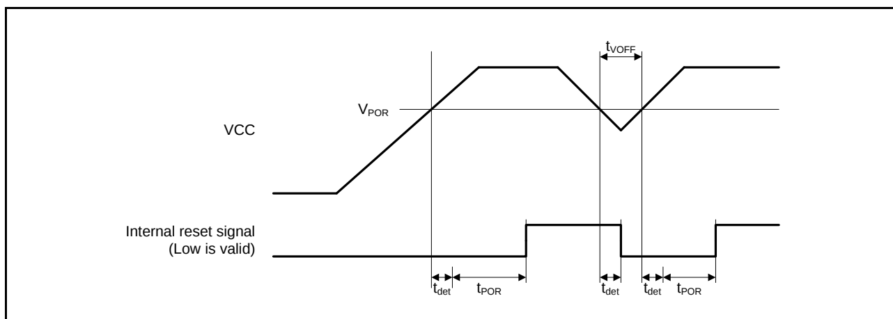
Figure 2.90 Power-on Reset Timing
