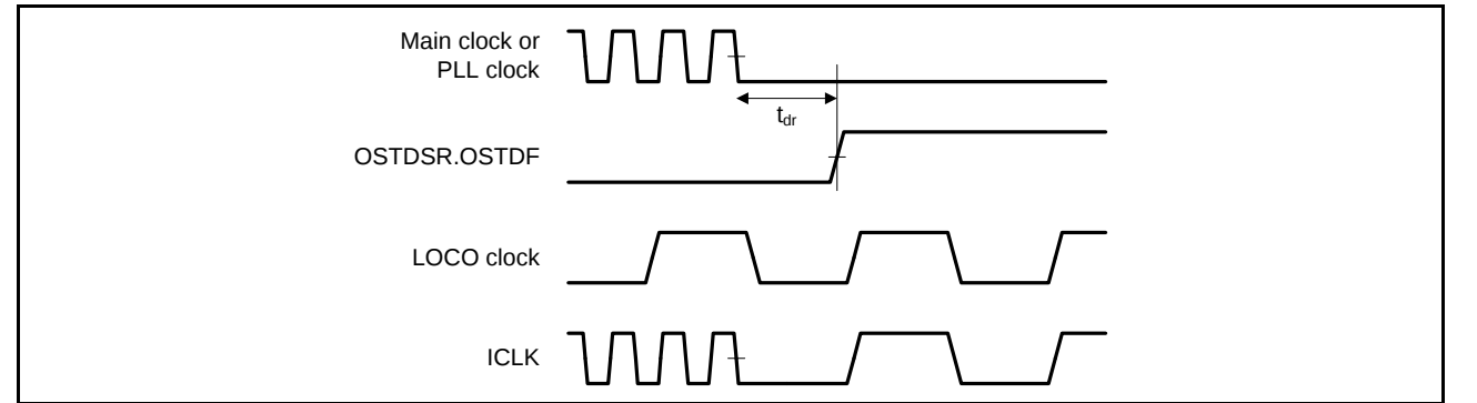
Figure 2.94 Oscillation Stop Detection Timing
