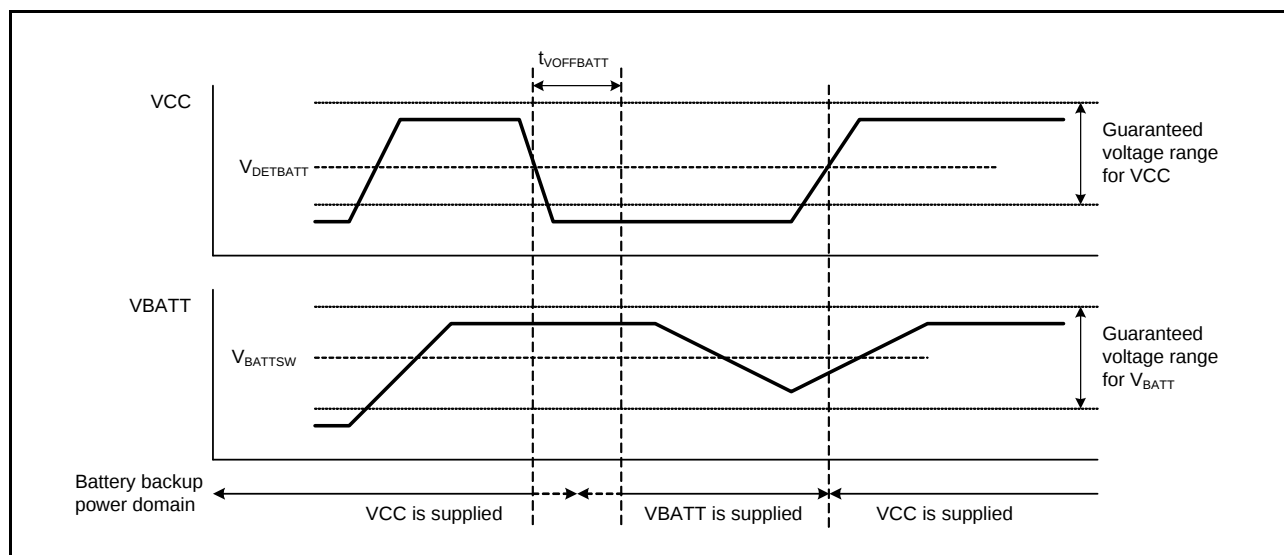
Figure 2.95 Battery Backup Function Characteristics
