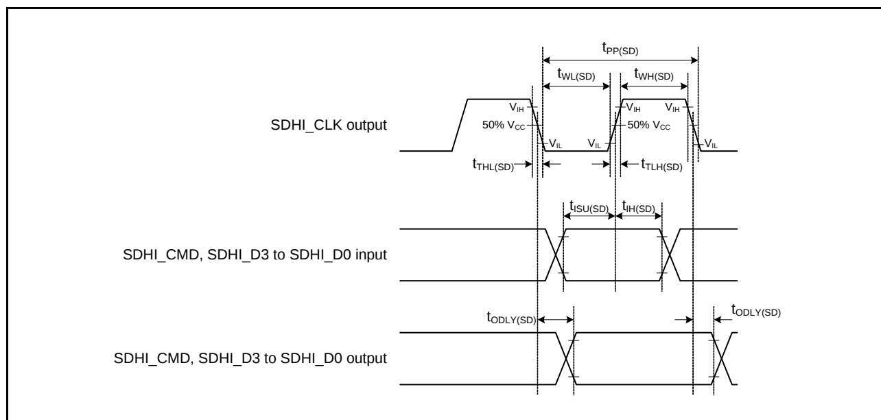
Figure 2.71 SD Host Interface Input/Output Signal Timing
