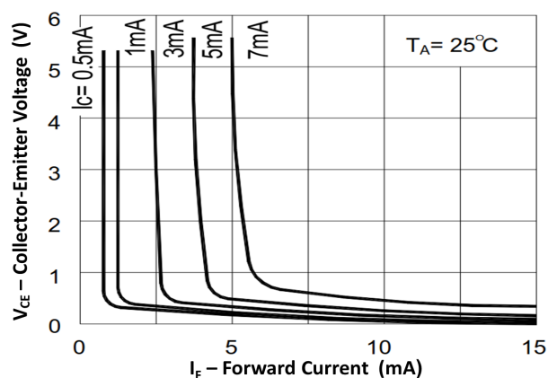
Fig 4 Collector-Emitter Voltage vs Forward Current
