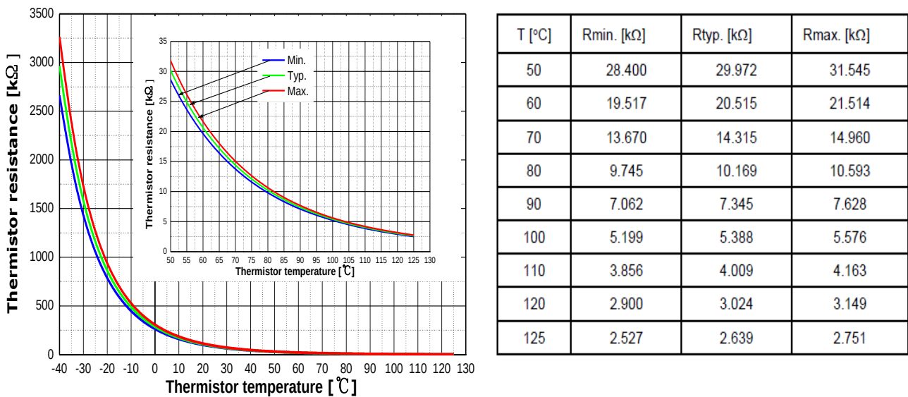
Figure 7 Thermistor resistance – temperature curve and table (For more information, please refer to the application note ‘AN CIPOS™-Mini 1 Technical description’)
