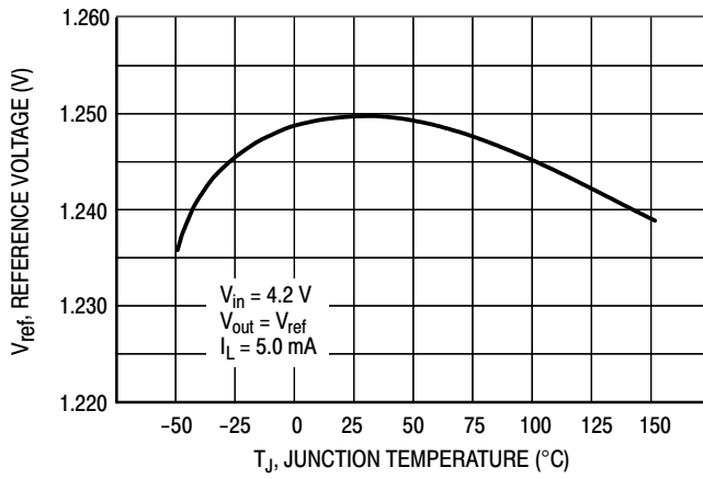
Figure 13. Temperature Stability
