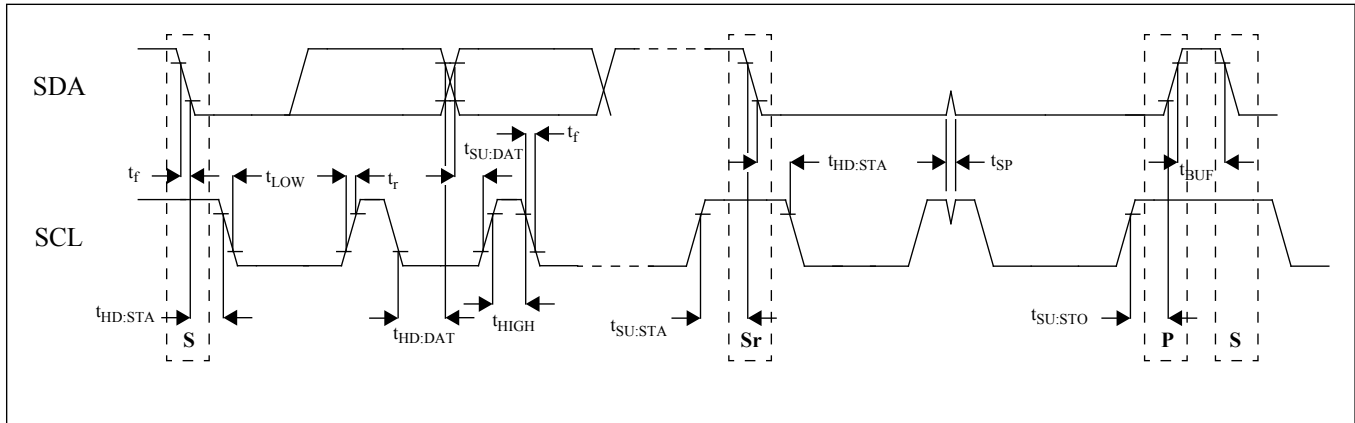
Figure 35 - I²C Serial Microport Timing
