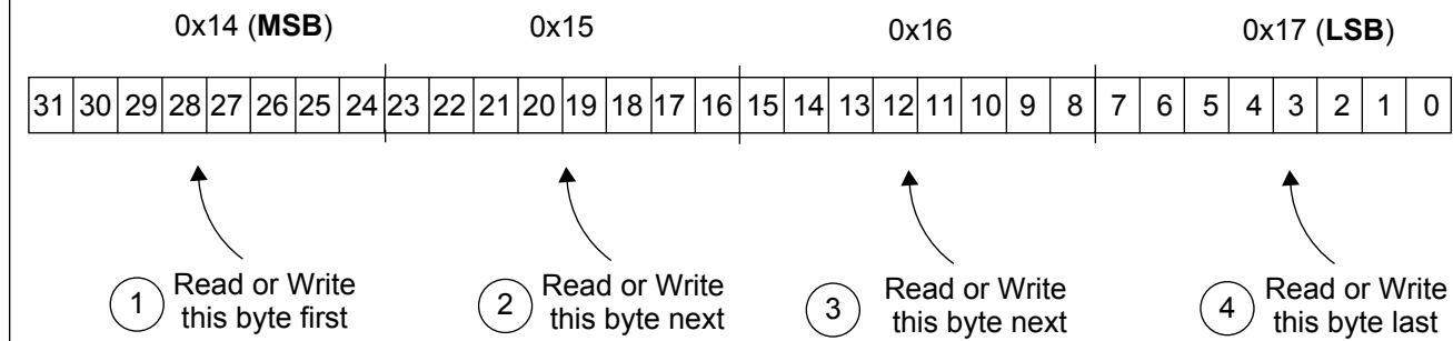
Figure 28 - Accessing Multi-byte Register Values
