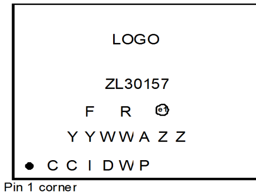
Figure 37 - Custom Factory Programmed Device Top Mark
