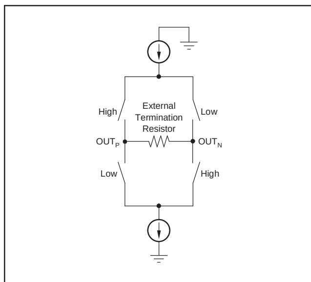
Figure 18. LVDS Buffer
