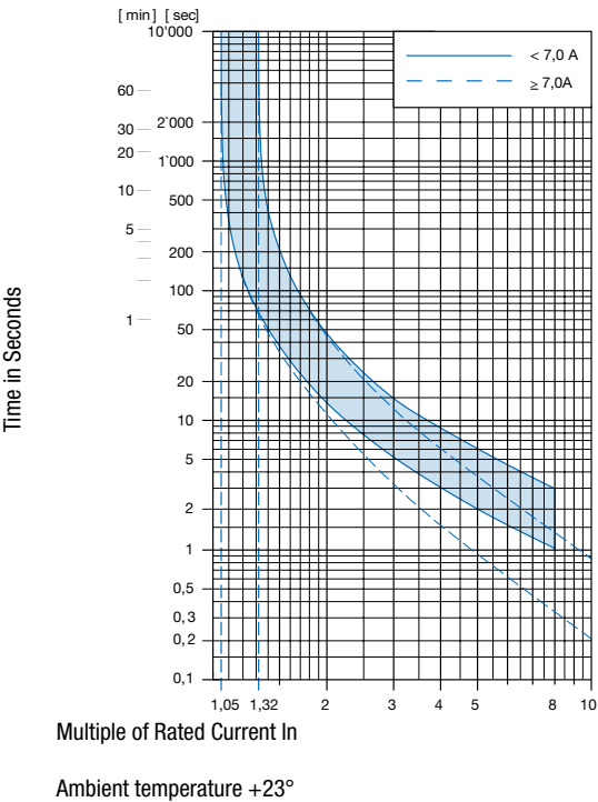
Time-Current-Curves
