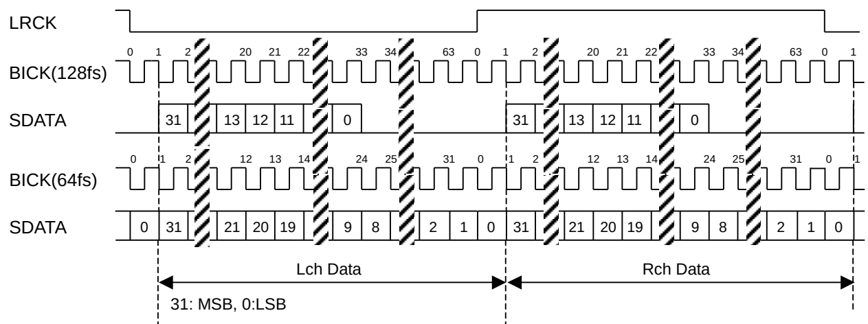
Figure 17. Mode 7 Timing
