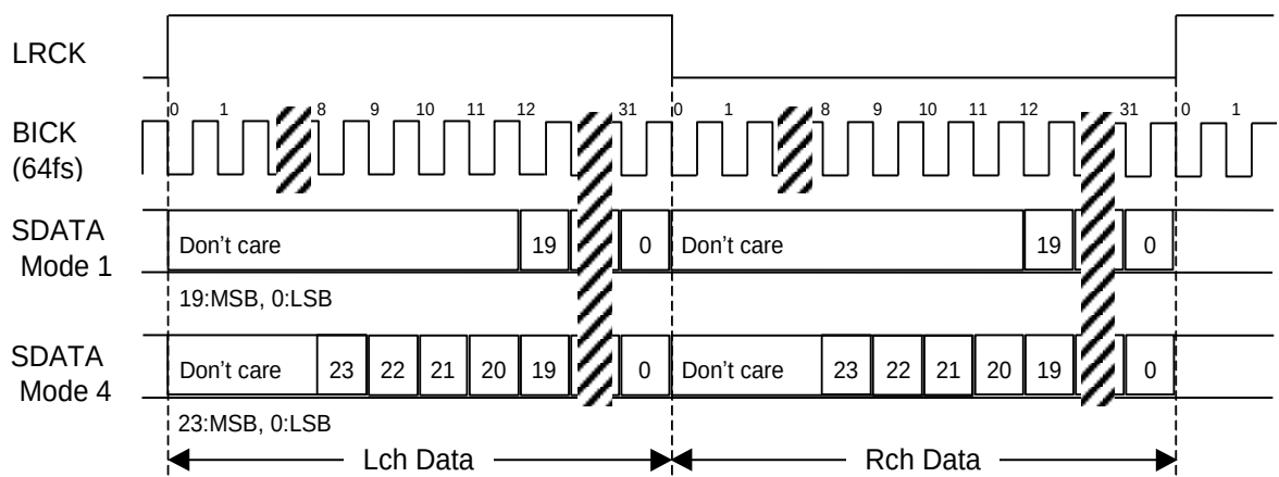
Figure 12. Mode 1/4 Timing
