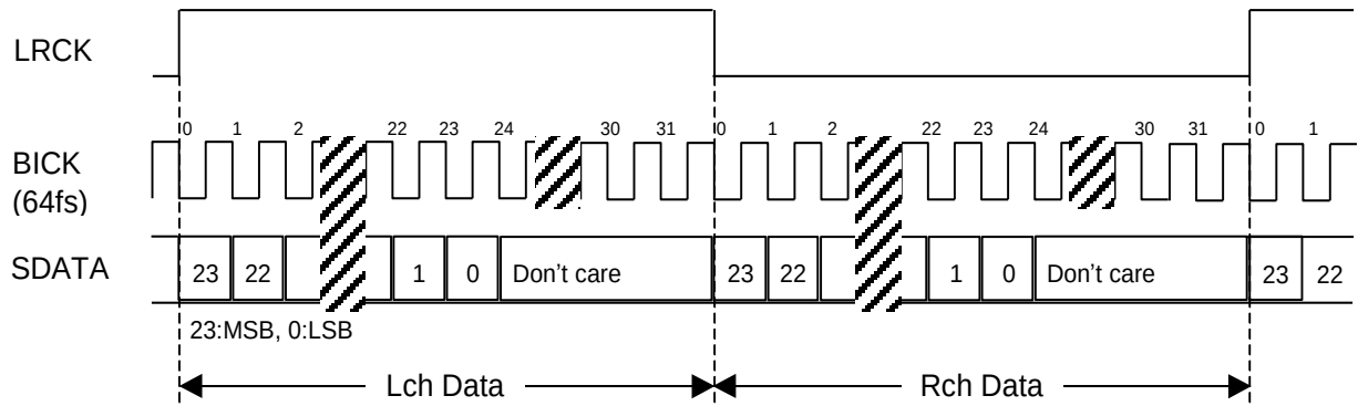
Figure 13. Mode 2 Timing
