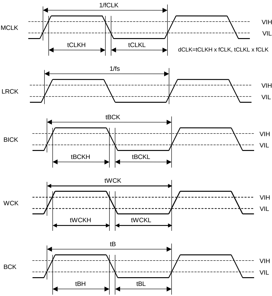
Clock Timing
