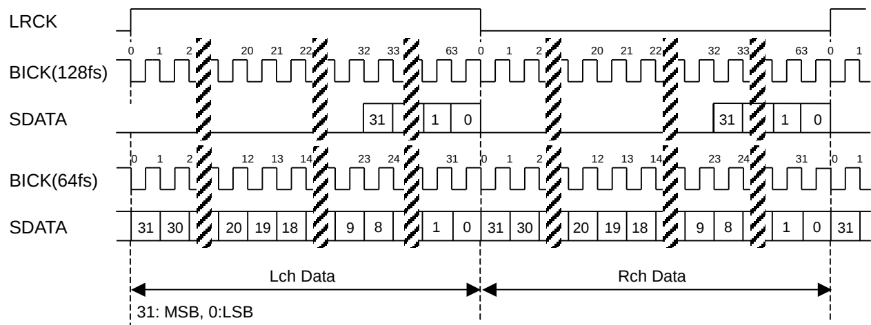
Figure 15. Mode 5 Timing
