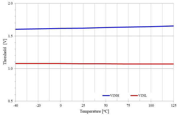
Figure 30. Input Logic Threshold vs. Temperature (INA, and INB)
