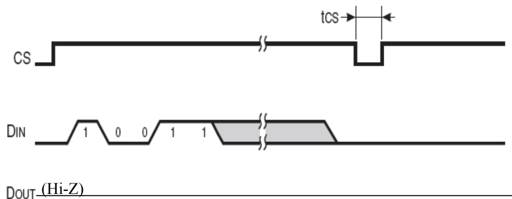
Fig. 4: Write Enable (WEN) Cycle Timing
