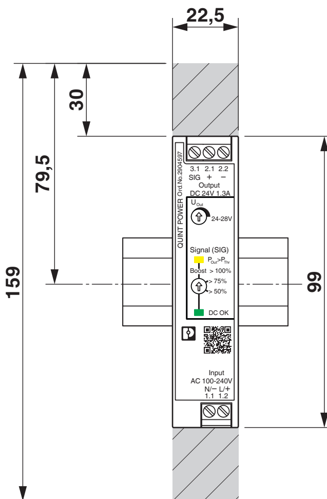
Dimensional drawing
