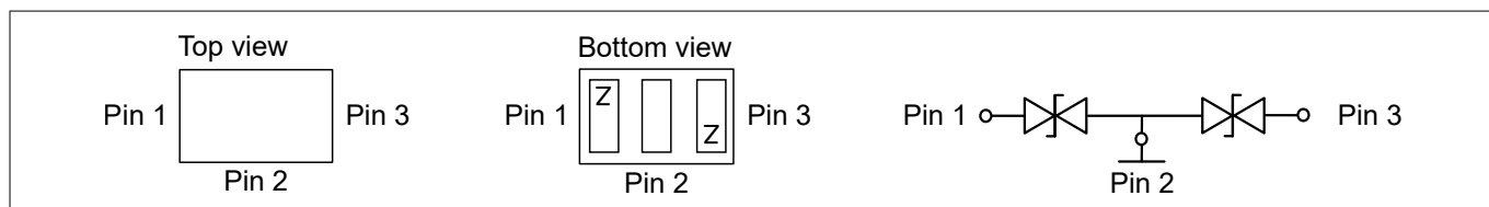
Figure 1 Pin configuration and schematic diagram
