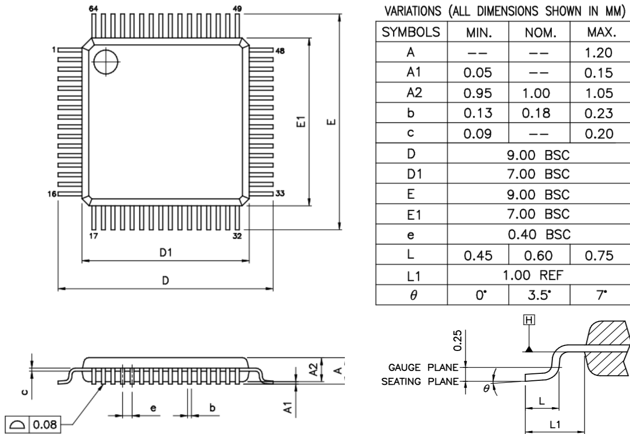
Figure 8-3 TQFP-64 Package Dimensions
