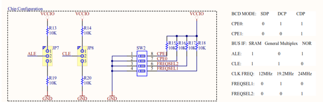
Figure 7-1 FT313H Chip Schematic
