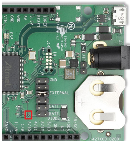
Figure 5: Resistor R9
