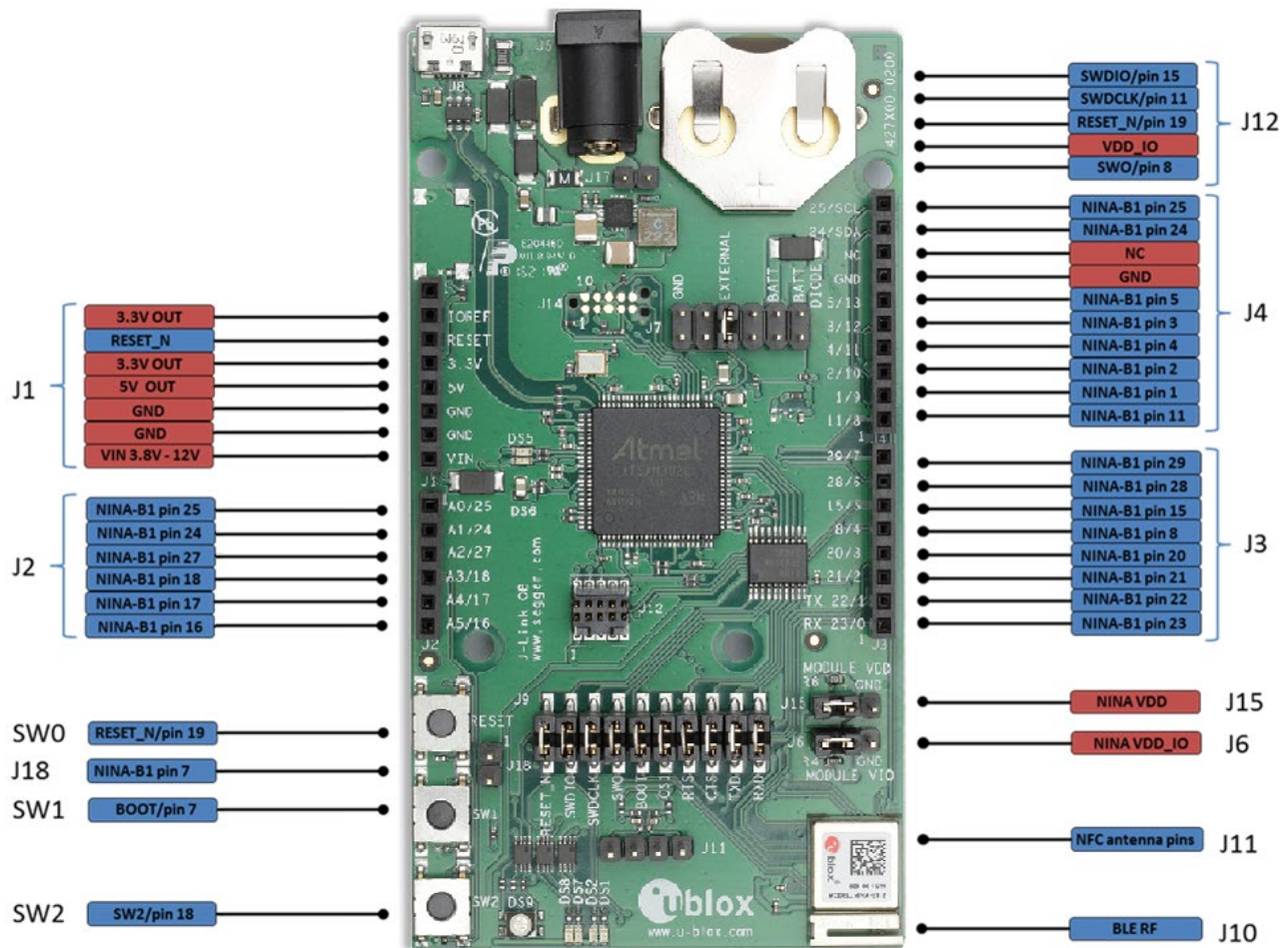
Figure 3: EVK-NINA-B1 connectors
