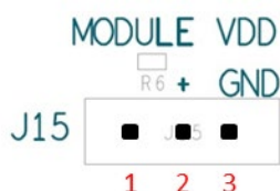
Figure 8: Current measurement pin header J15 of EVK-NINA-B1
