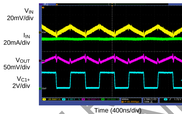
Output Ripple (AP3606, V_{IN}=3.3\text{V} , I_D=80\text{mA} )
