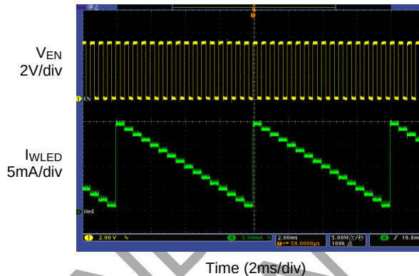
1x Mode Dimming Operation (AP3607, V_{IN}=5\text{V} , f_{EN}=2\text{kHz} )
