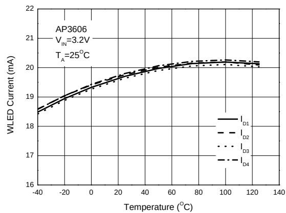
1.5x Mode WLED Current vs. Temperature
