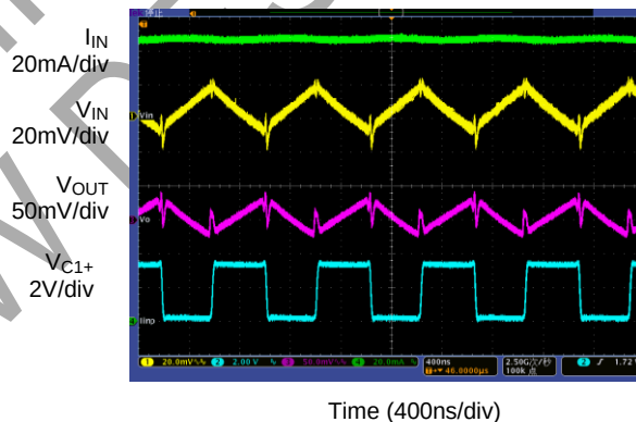
Output Ripple (AP3607, V_{IN}=3.3\text{V} , I_D=120\text{mA} )
