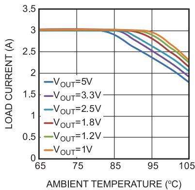
Thermal Derating
