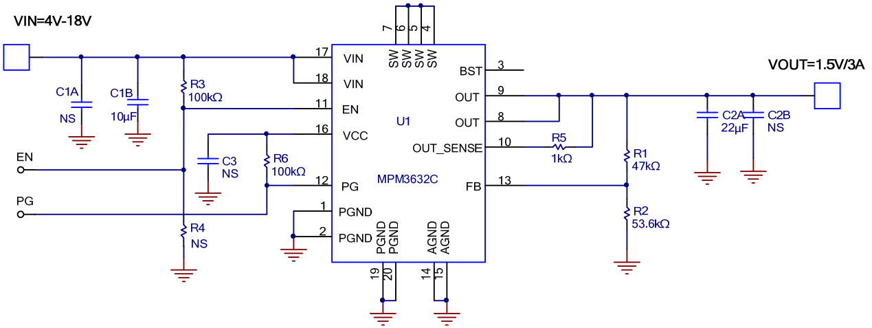
Figure 12: 1.5V Output
