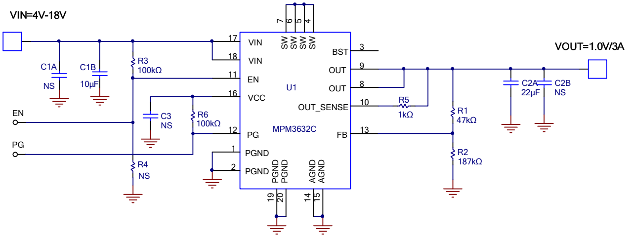
Figure 14: 1.0V Output
