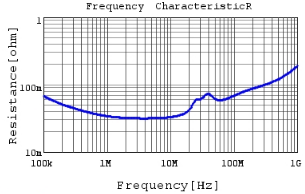
RDER71H334K1P1H03B R DCOV, 25degC
