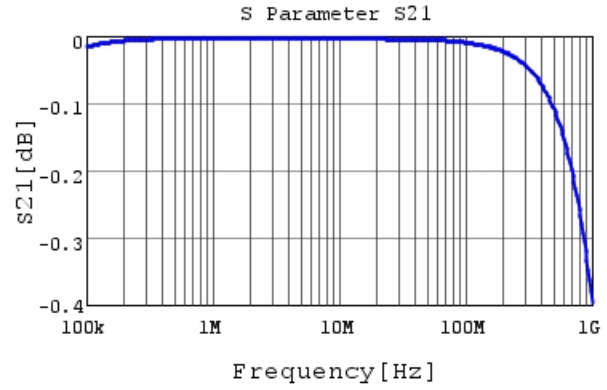
RDER71H334K1P1H03B S21 DC0V, 25degC
