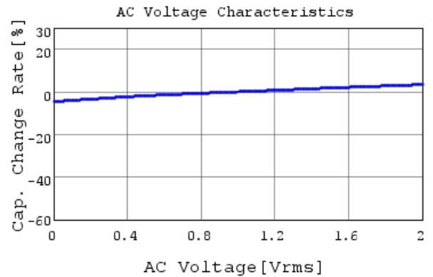
RDER71H334K1P1H03B C-AC Voltage capchange, I
