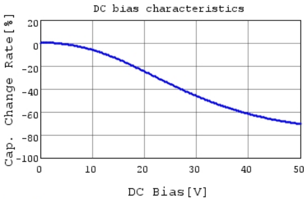
RDER71H334K1P1H03B C-DC bias capchange, 25.0
