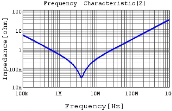
RDER71H334K1P1H03B |Z| DCOV, 25degC
