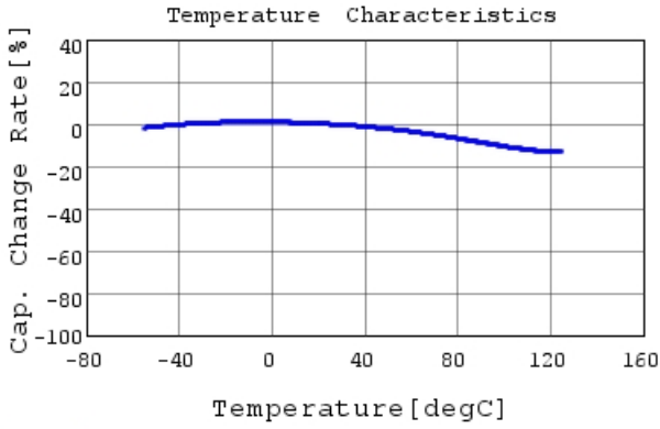
RDER71H334K1P1H03B C-Temp. capchange, DC0.0V
