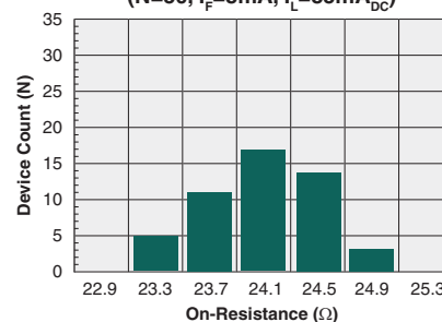
Typical On-Resistance Distribution (N=50, I_F=8\text{mA} , I_L=85\text{mA}_{DC} )
