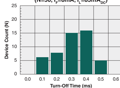
Typical Turn-Off Time (N=50, I_F=8\text{mA} , I_L=85\text{mA}_{DC} )
