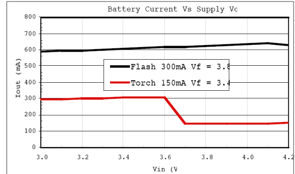
Fig. 17: Battery Current vs Supply Voltage D1=AOT3228HPW0303B LED, R_{SENSE}=0.3\Omega R_{SET}=140k\Omega , C_{IN}=2.2\mu F , C_{FC}=0.47\mu F , C_{OUT}=1\mu F
