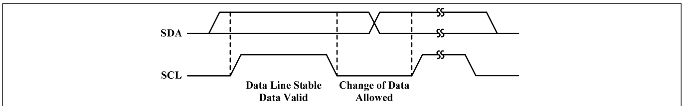
Figure 4 Bit Transfer
