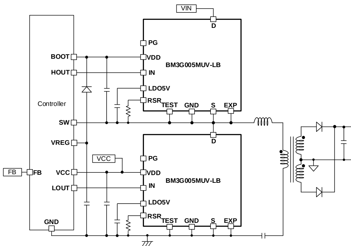
Figure 6. LLC Resonant Converter Application Example
