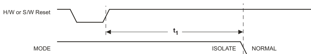
Figure 9-23. Isolation Timing
