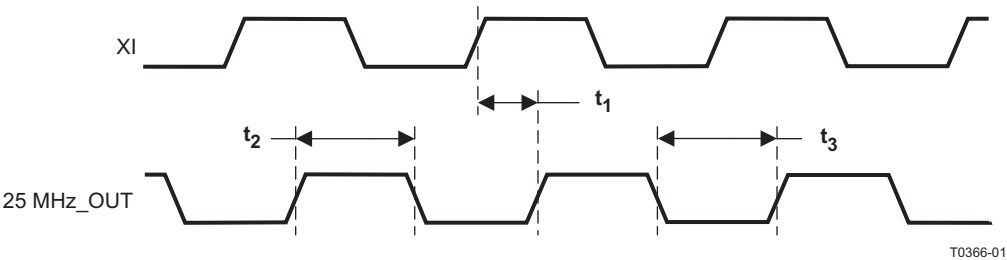
Figure 9-24. 25 MHz_OUT Timing
