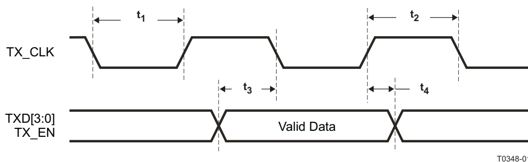
Figure 9-11. 10 Mb/s MII Transmit Timing
