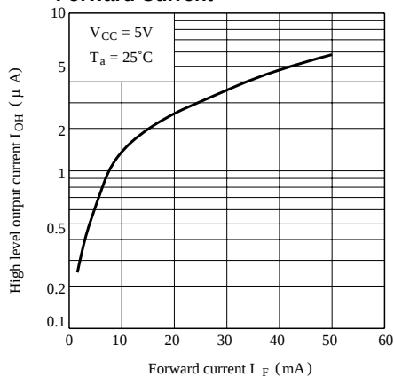
Fig. 8 High Level Output Current vs. Forward Current
