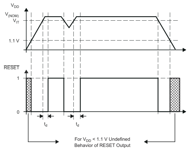
Figure 7-1. Timing Diagram
