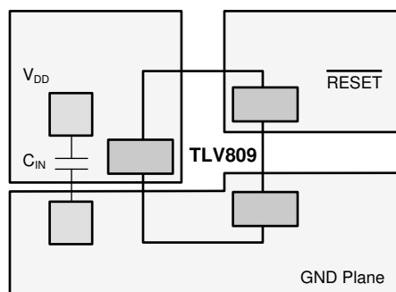
Figure 11-1. Example Layout
