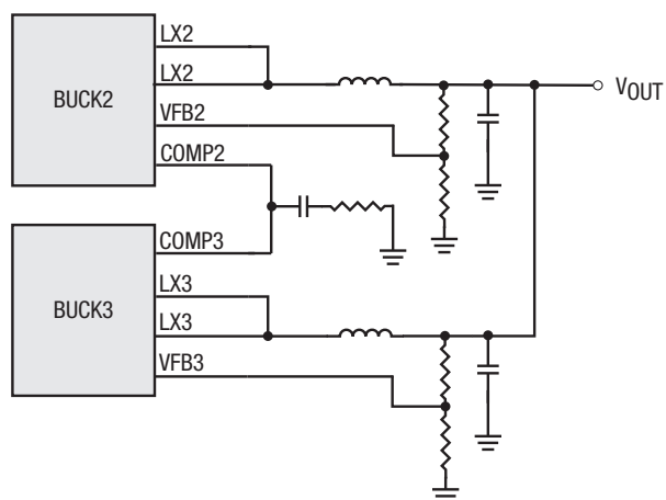
Figure 31. Parallel Operation
